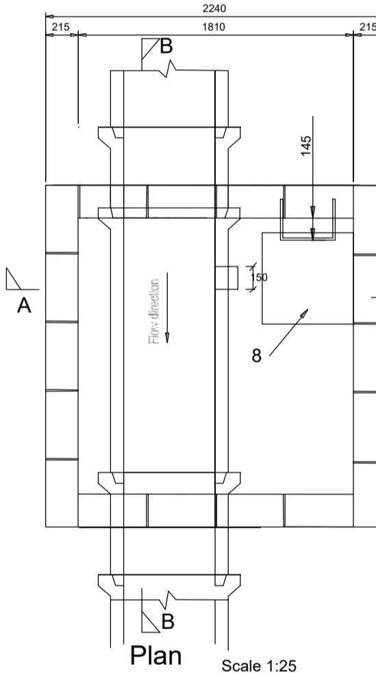
Plan
