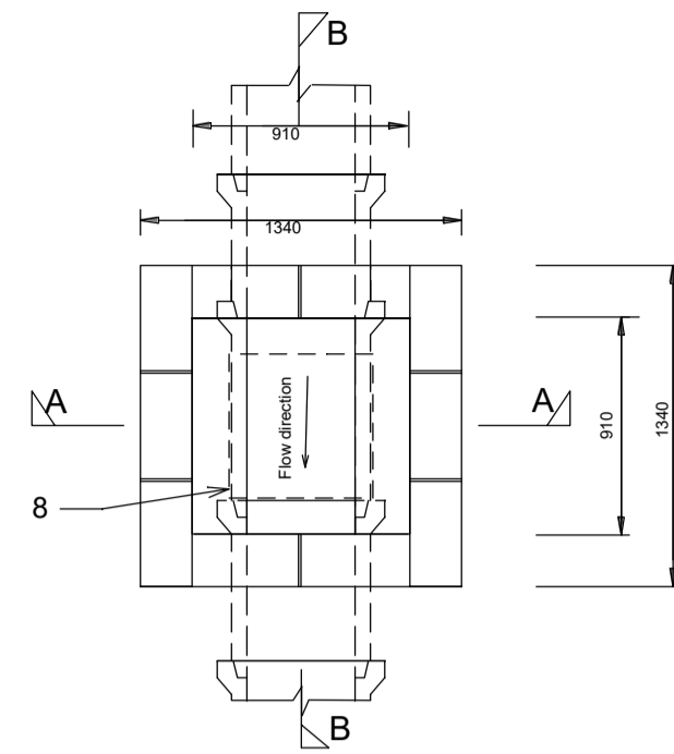
Plan Below Roof Slab
