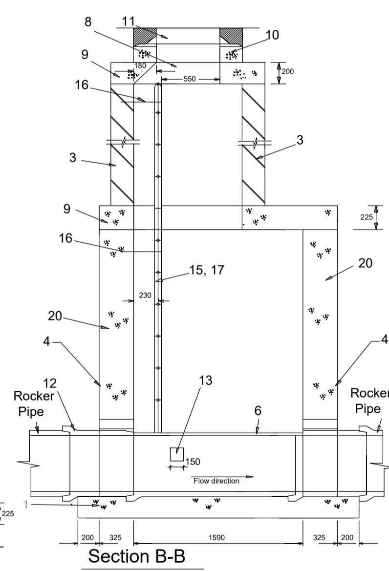
Section B-B
